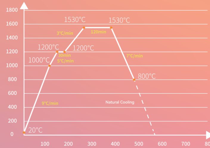
Prisma (1-3 unit ) bridge sintering curve
