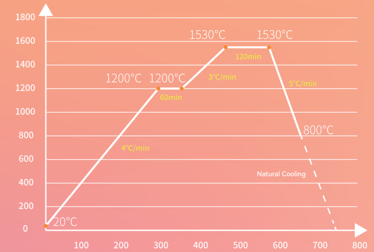
Prisma (4-6 unit ) bridge sintering curve
